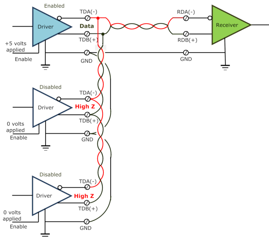
Figure 9: Tri-State Control
