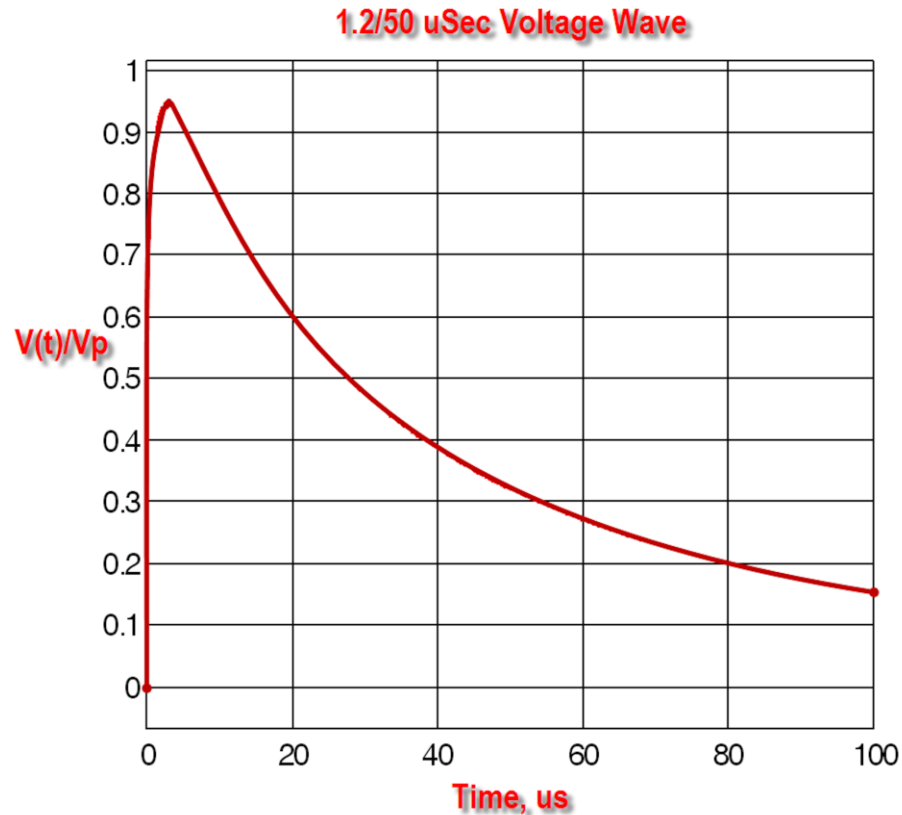
Figure 35: Combination Wave Voltage Waveform
