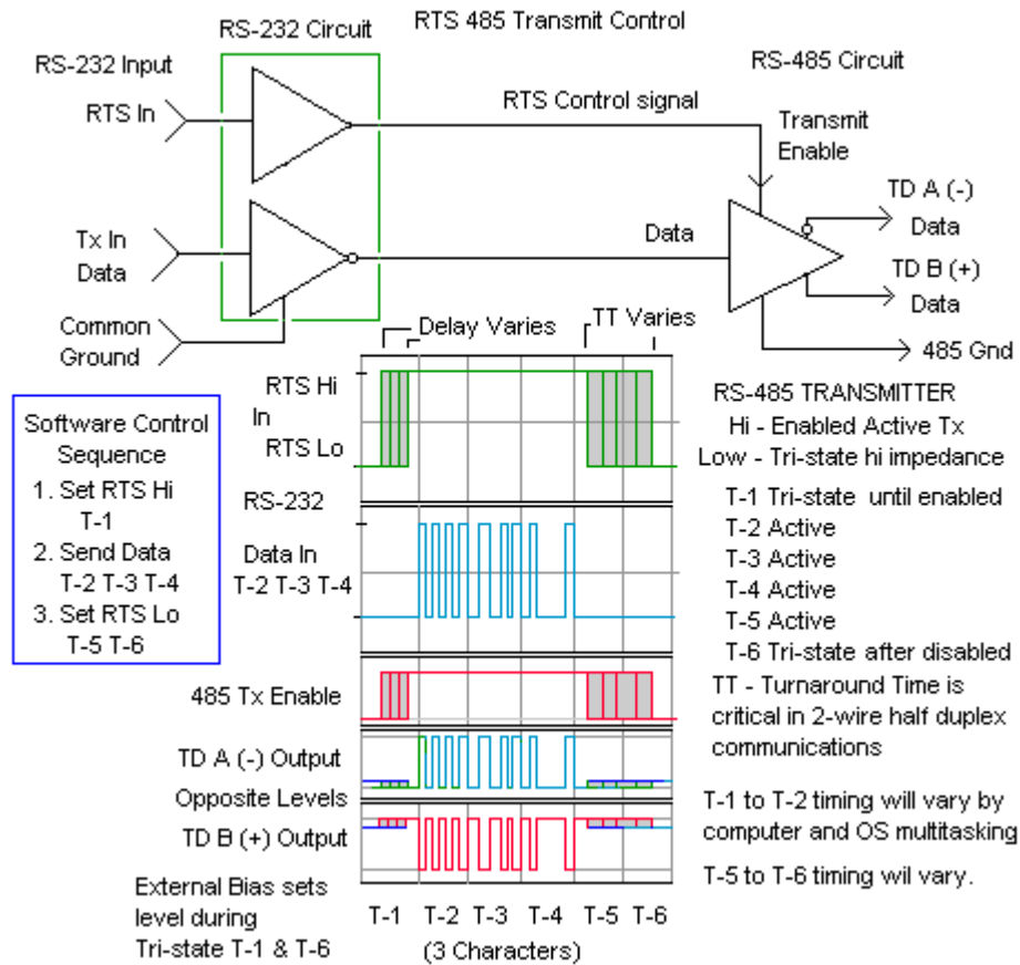
Figure 63: RTS Timing
