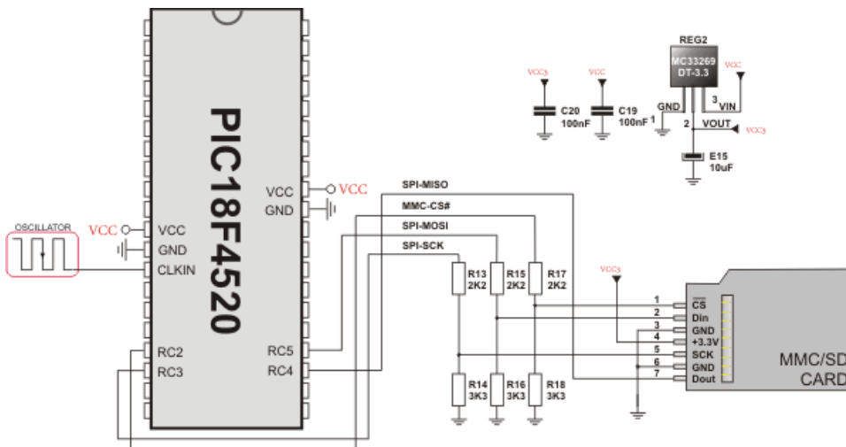
MMC interface
