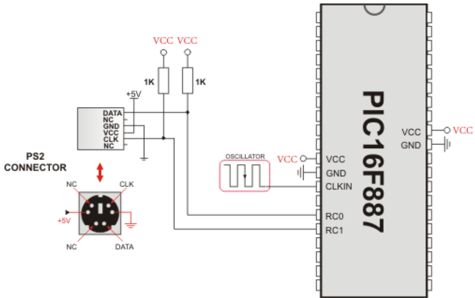
Example of PS2 keyboard connection
